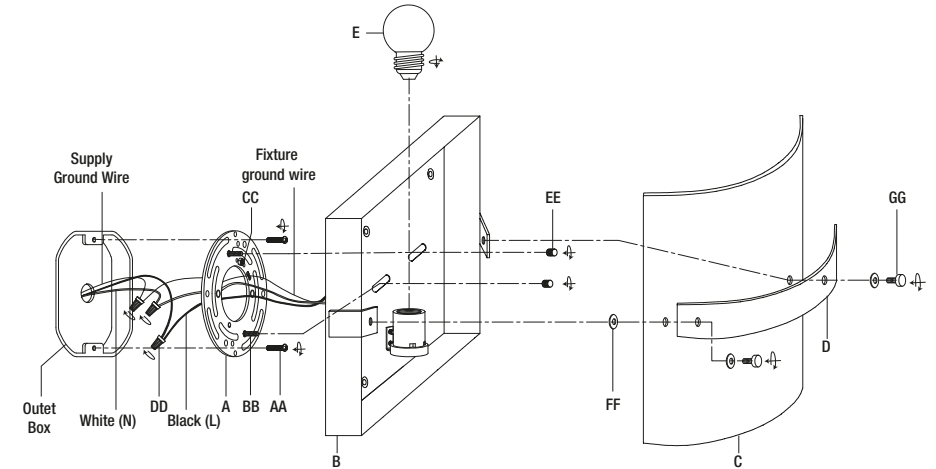
AA - Outlet Box Screw (x2)
